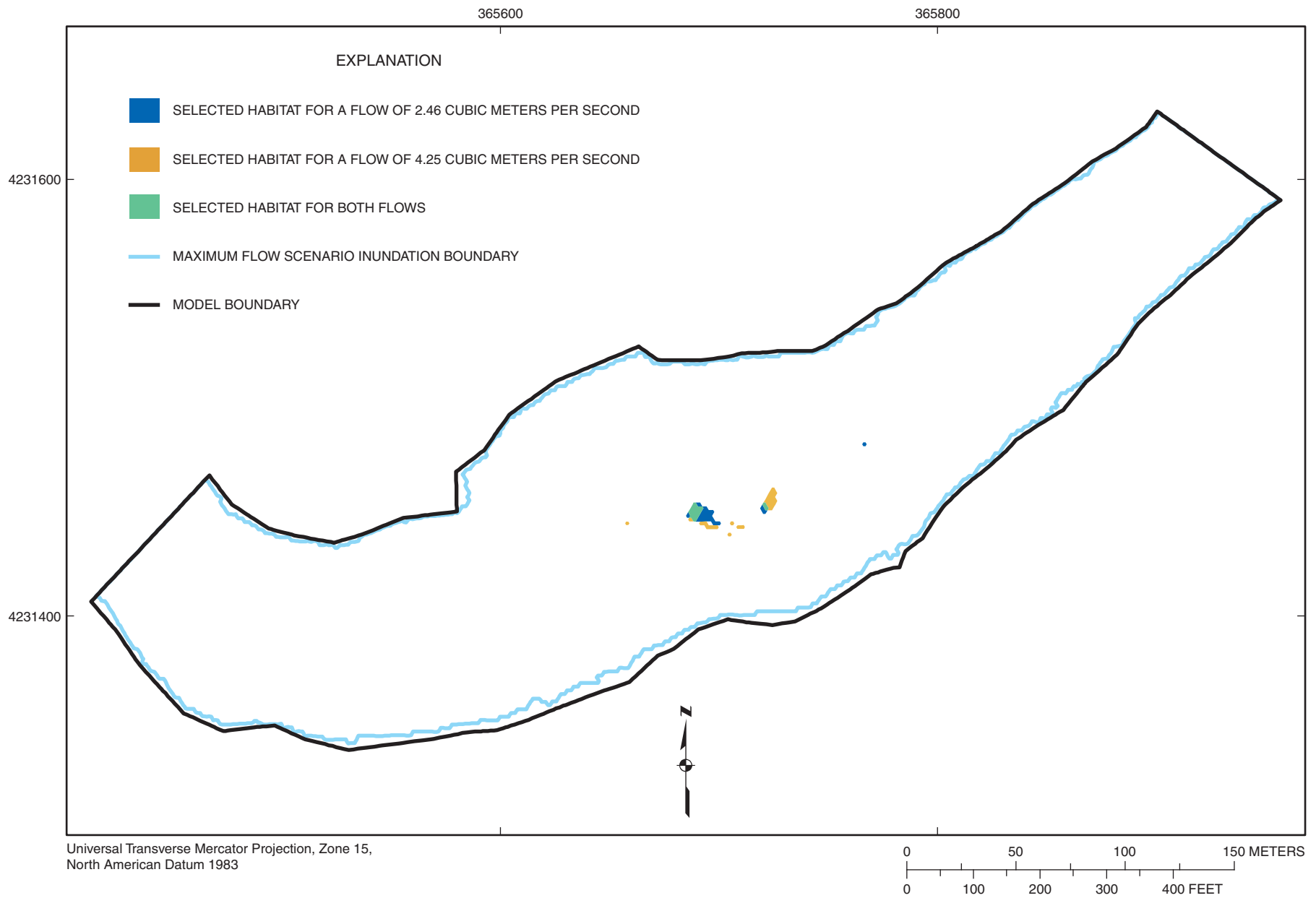
Figure 4-69. Selected habitat area distribution for habitat category 19 (stonecat) at flows of 2.46 and 4.25 cubic meters per second at Marais des Cygnes River site MDC2.
